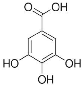
Figure 2.1: Gallic Acid
